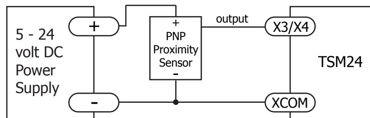
Connecting a PNP type Proximity Sensor to an Input
