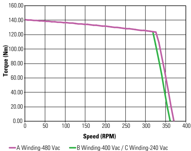
KBM(S)-79X03 ContinuousTorque
