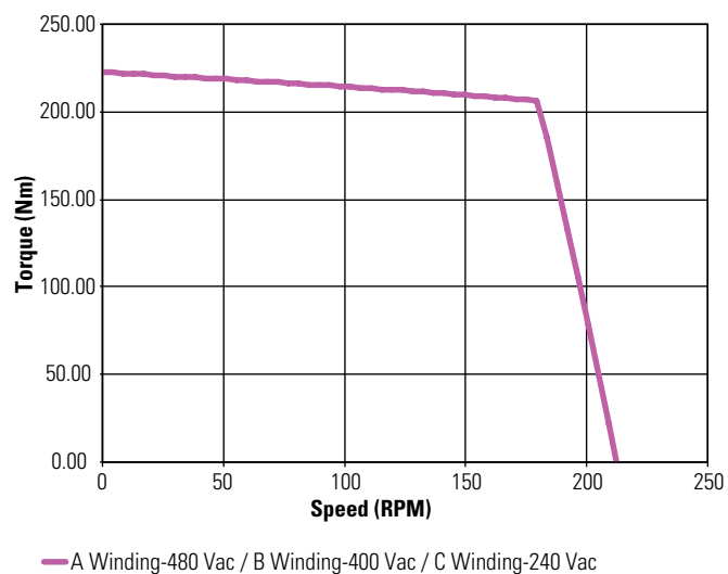
KBM(S)-79X05 Continuous Torque
