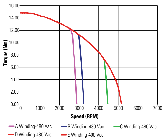
KBM(S)-25X04 ContinuousTorque
