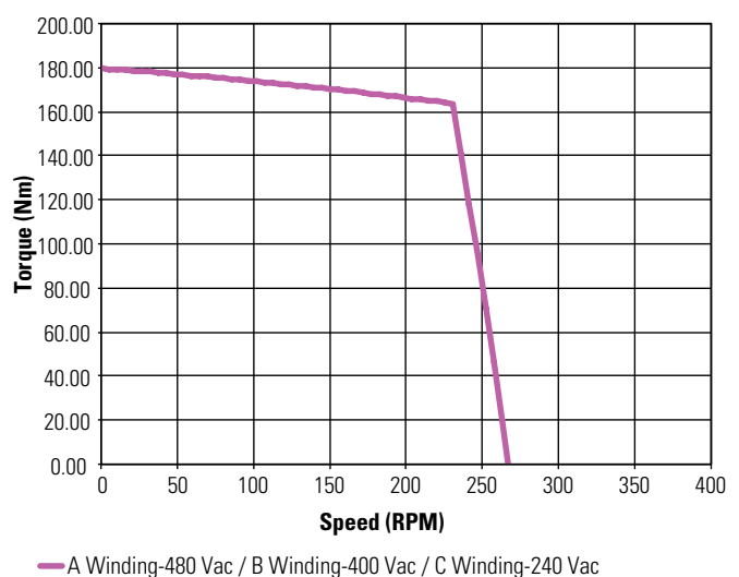
KBM(S)-79X04 ContinuousTorque
