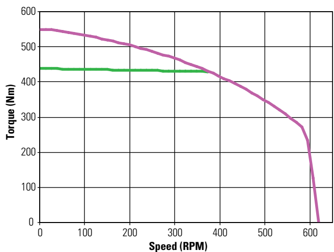
KBM(S)-118X03 ContinuousTorque
