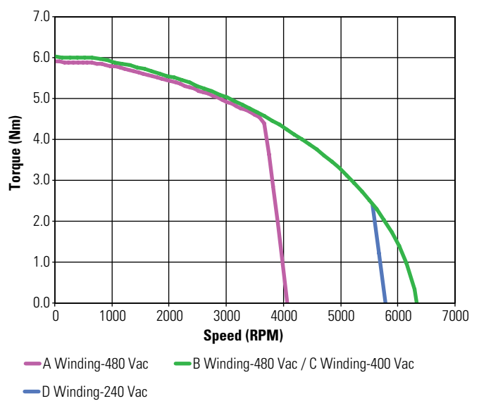
KBM(S)-17X04 Continuous Torque
