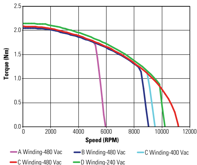
KBM(S)-14X02 Continuous Torque
