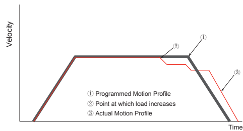
Figure 2: Diagram showing the Stall Prevention process
