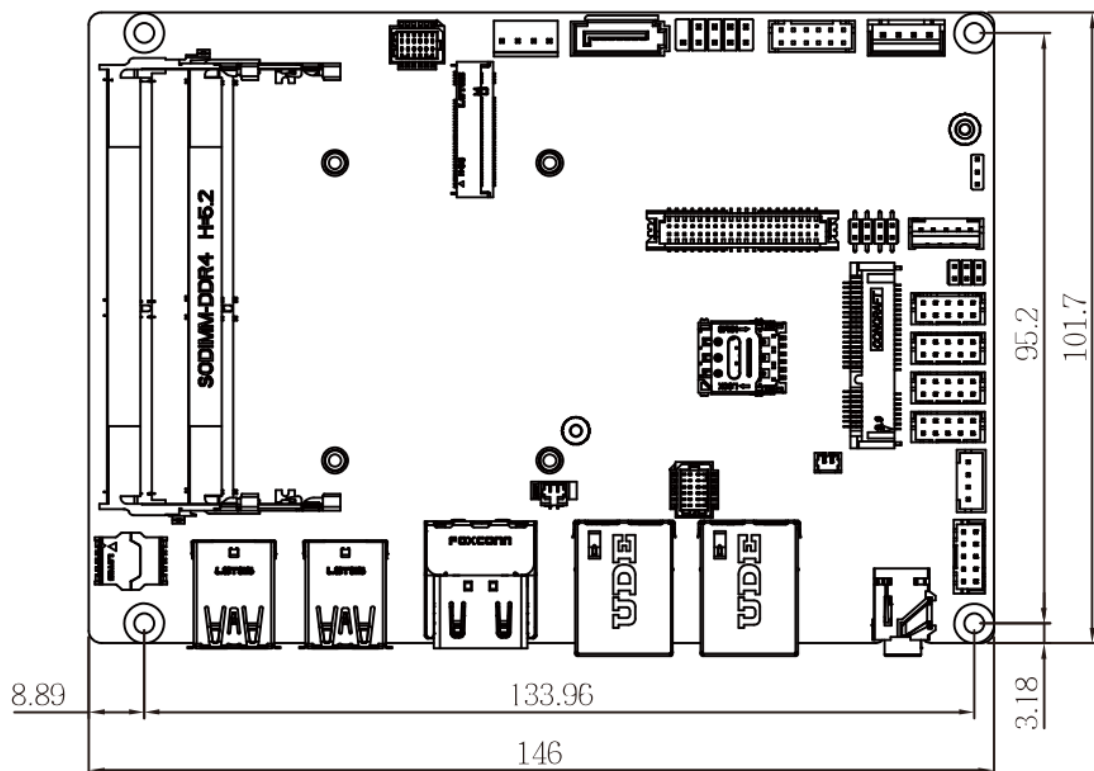
Figure 2.1: Motherboard Dimensions
